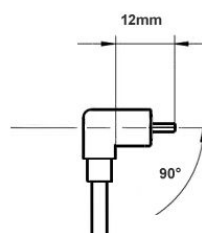
USB 2.0 MICRO B 90°
