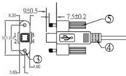
USB 2.0 B plug A110-507-001
