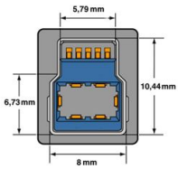
USB 3.0 B
