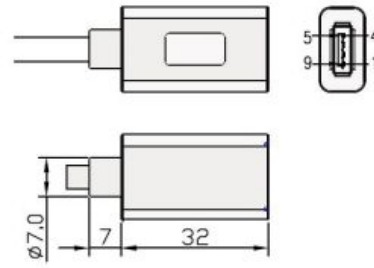
USB 3.0 A female
